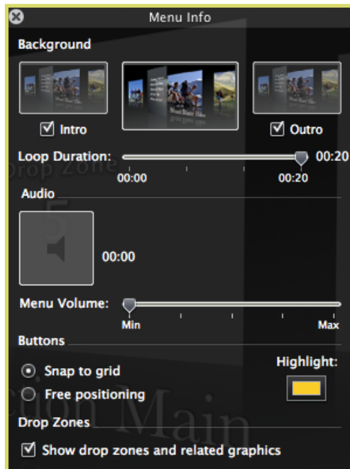
Figure 16. Inspector Window
