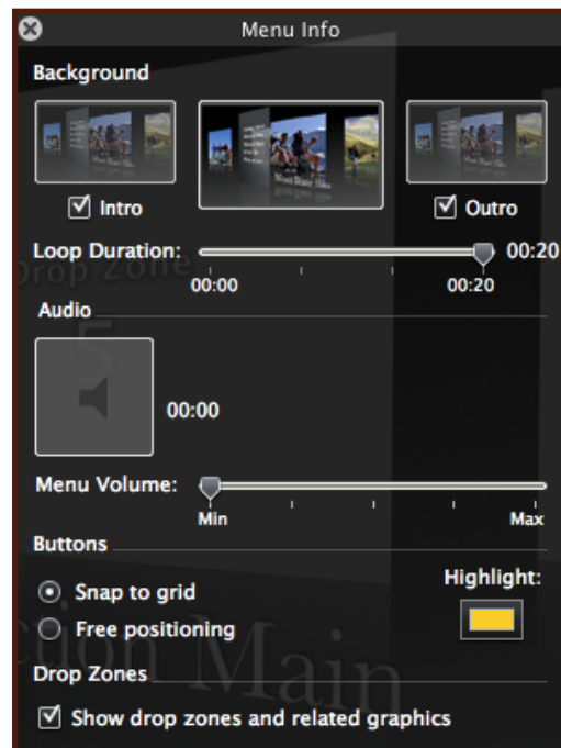
Figure 16. Inspector Window
