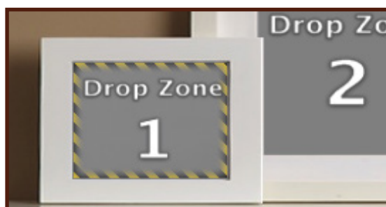
Figure 10. Drop Zone
