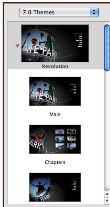
Figure 8. Theme Tab
