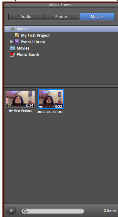
Figure 4. Media Browser
