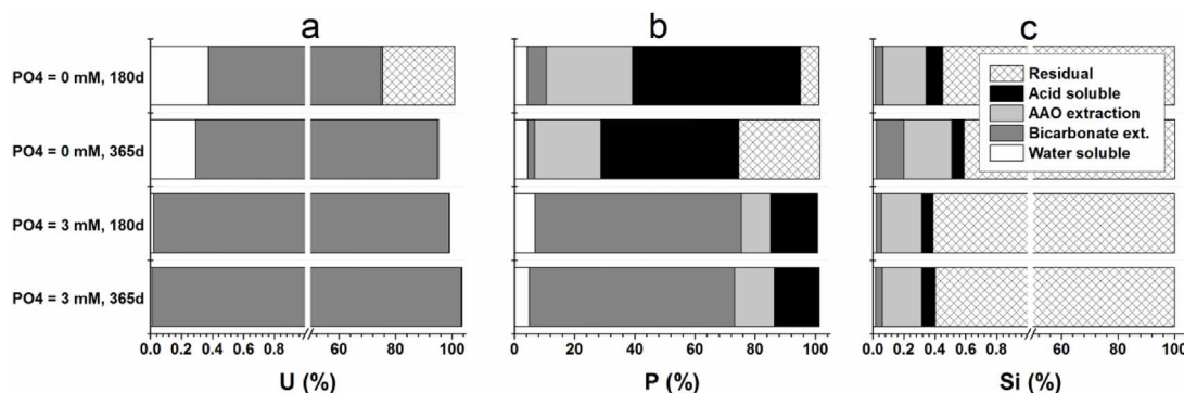
Fig. 6. Percentage of total U, P, and Si released during sequential extraction. Sequential extractions were only performed on the sediments reacted with 0.86 mM U.
