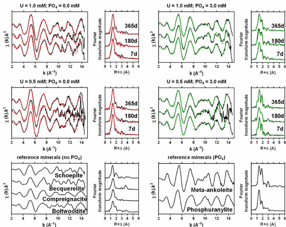
Fig. 5. U L III edge EXAFS spectra and corresponding Fourier transform of model uranium compounds (bottom) from Kanematsu et al. (2014) and sediments reacted for 7, 180 and 365 days under the different treatments. Black lines represent the experimental spectra and dotted colored lines are the results of linear combination fits reported in Table 2.
