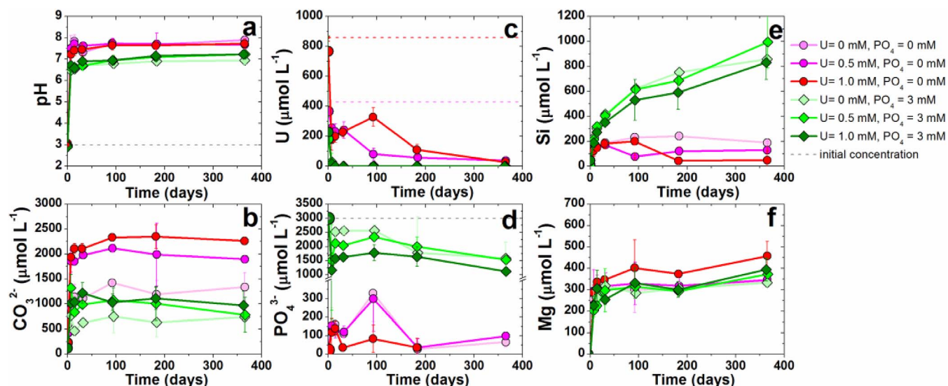
Fig. 1. Evolution of solution chemistry during reaction for pH (a), Total inorganic carbon reported as \text{CO}_3^{2-} (b), U (c), total \text{PO}_4^{3-} (note the break on the y-axis) (d), Si (e) and Mg (f). Note the y-axis break for panel d.
